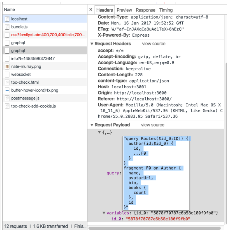
Relay GraphQL Call in Network Pane
