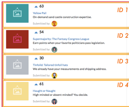
Product components inside of the ProductList component
