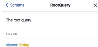
Server Docs
