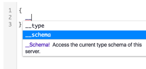
Server Introspection
