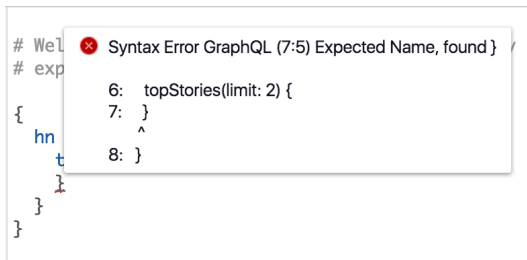
GraphiQL error without scalar
