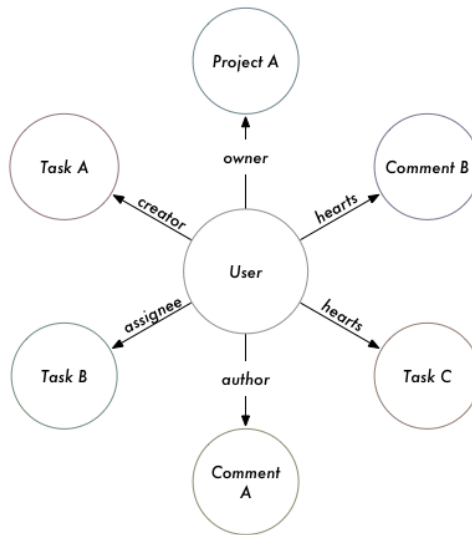
Asana Graph
