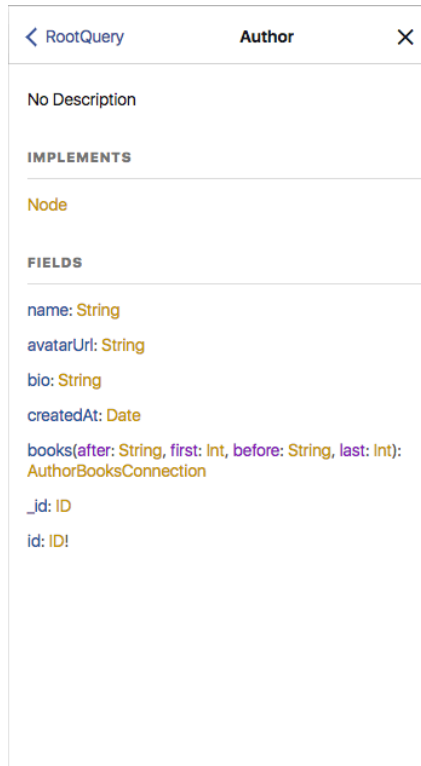
GraphQL Author Type
