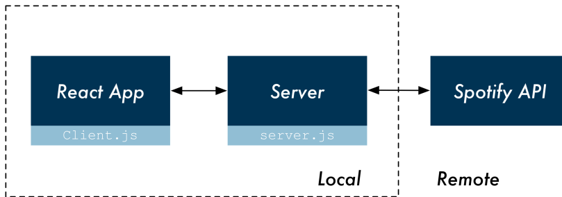
Communication diagram
