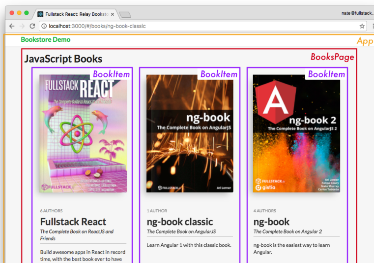
Books Page Components
