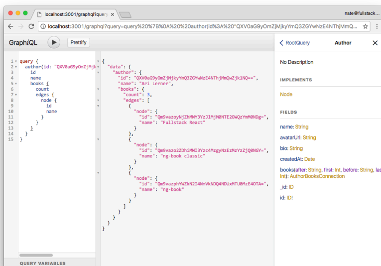
GraphQL Author with Books
