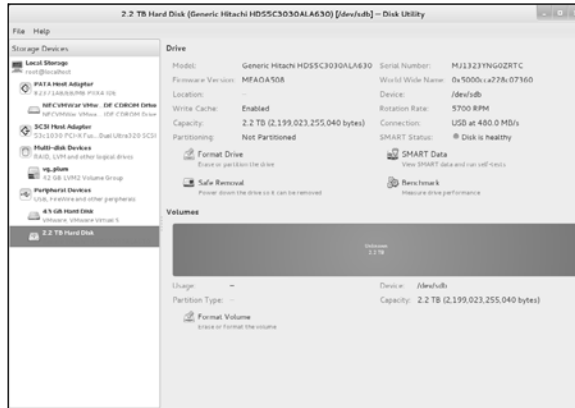
Figure 3-23 A disk without a partition table
