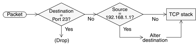
Figure 25-1 Example of how rules work
