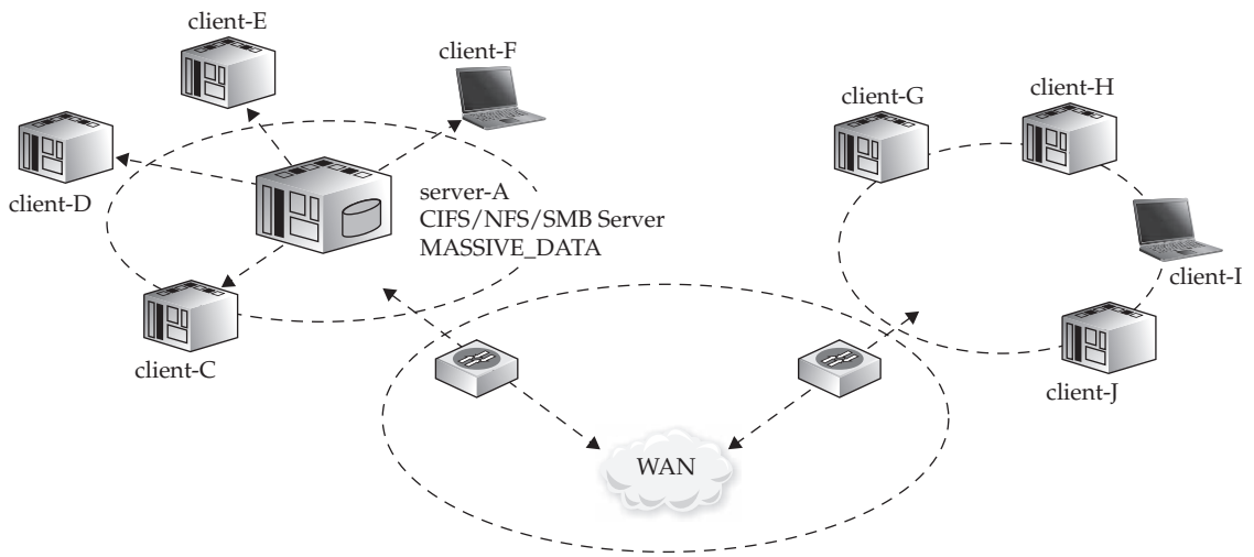
Figure 25-2 Traditional network file server, LAN clients, and WAN clients
