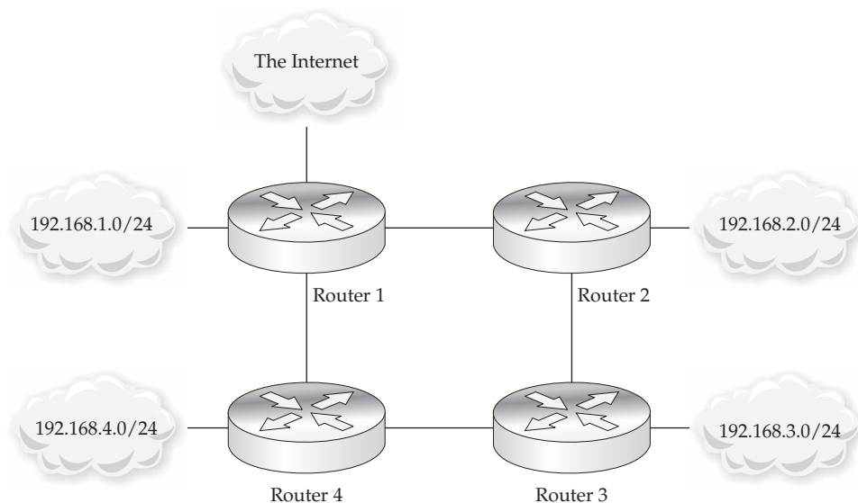
Figure 11-10 A small campus network using RIP
