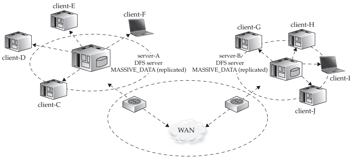
Figure 25-3 Distributed File Systems network
