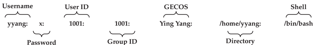
Figure 5-1 Fields of the /etc/passwd file
