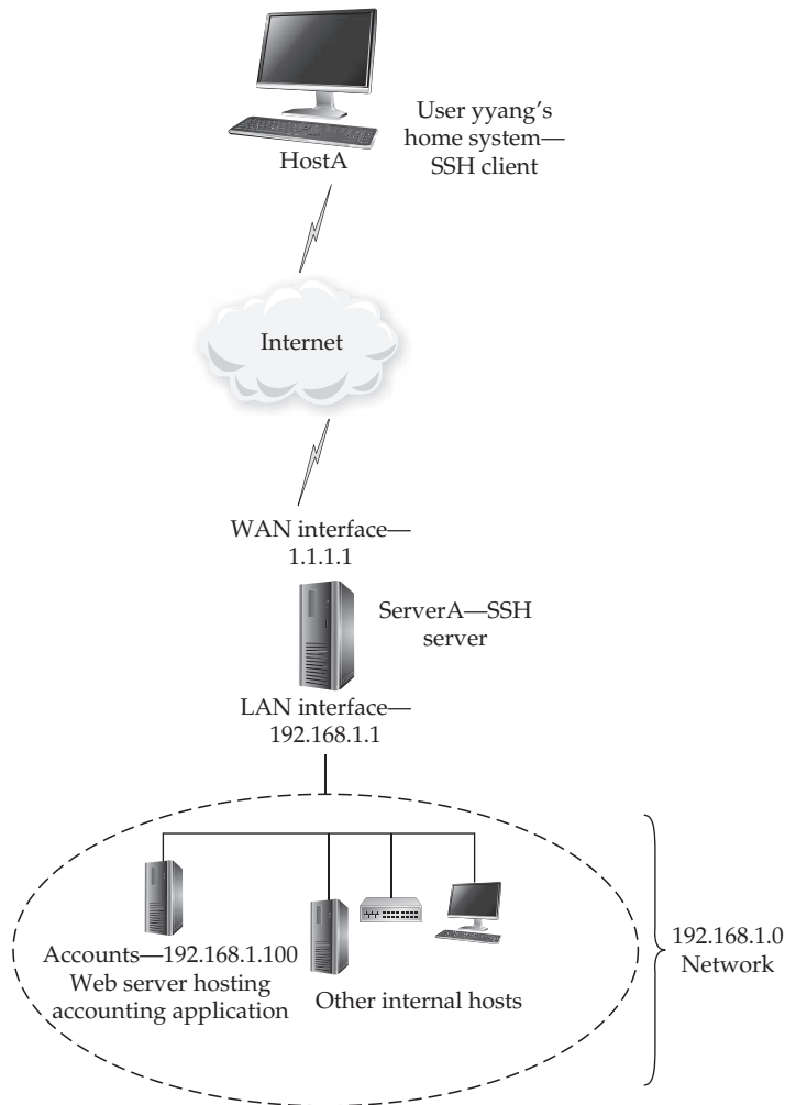
Figure 22-5 Port forwarding with SSH
