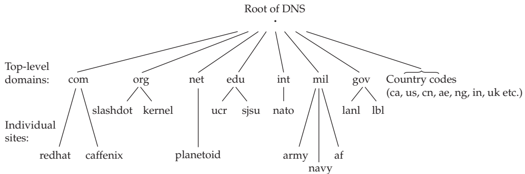
Figure 16-2 The DNS tree, two layers deep
