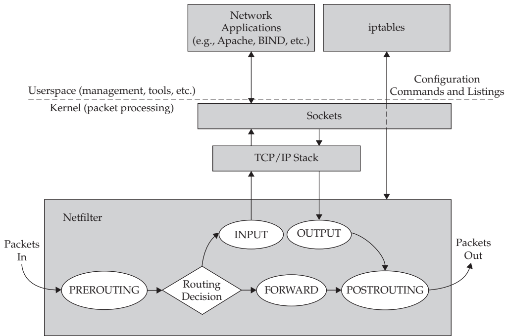
Figure 13-3 The relationship between the predefined chains in Netfilter
