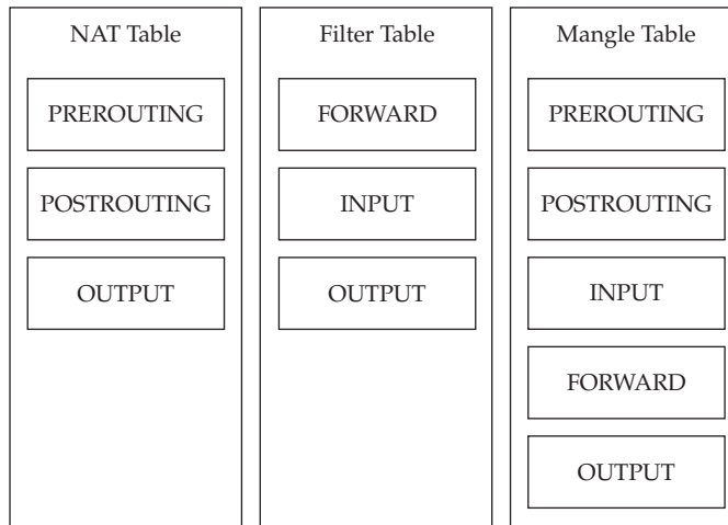
Figure 13-4 The relationship among predefined chains and predefined tables
