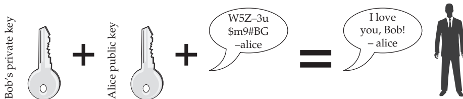
Figure 22-4 Bob uses Alice's public key, along with his private key, to verify and decrypt the data, respectively.
