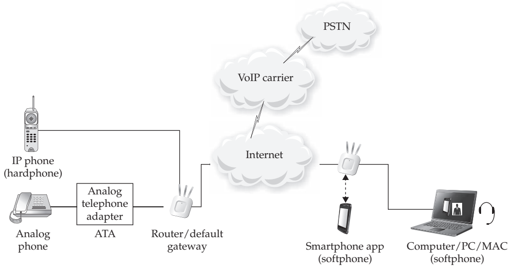
Figure 21-2 VoIP network layout using an ATA and IP phones
