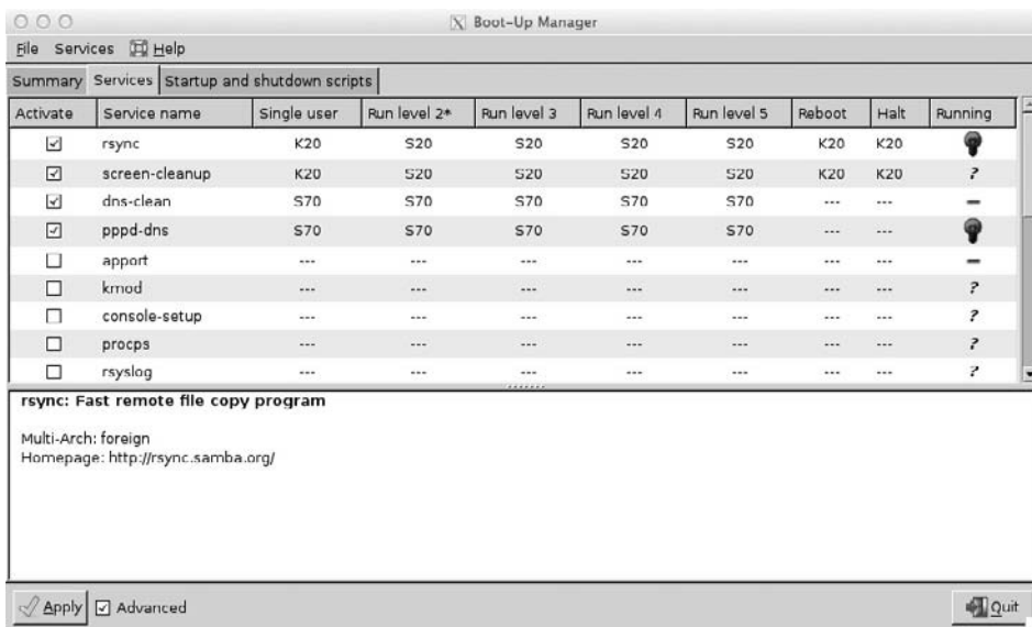
Figure 6-4 Ubuntu's Boot-Up Manager
