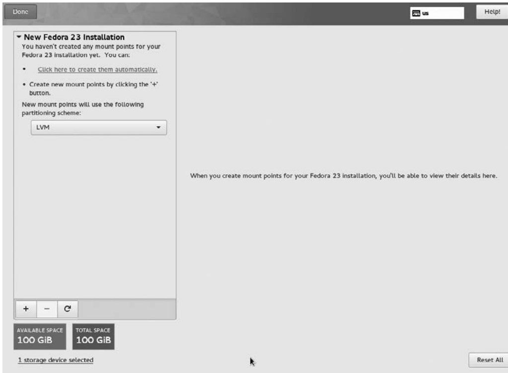
Figure 2-2 Manual Partitioning screen
