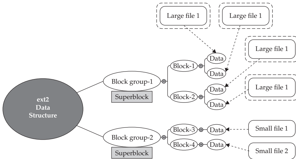
Figure 7-2 Data structure on ext2 file systems
