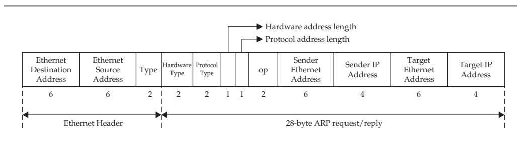
Figure 11-8 The ARP packet header
