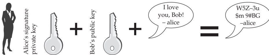
Figure 22-2 Alice uses Bob's public key, along with her private key, to encrypt and sign the data, respectively.
