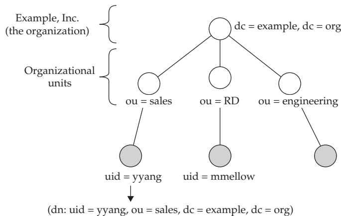
Figure 27-1 LDAP tree for example.org
