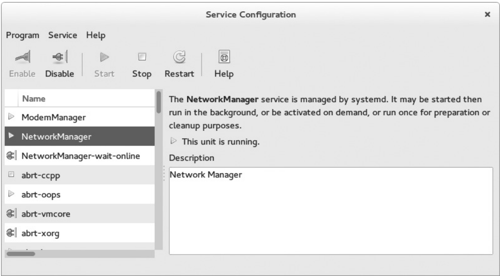
Figure 6-1 Fedora’s Service Configuration tool
