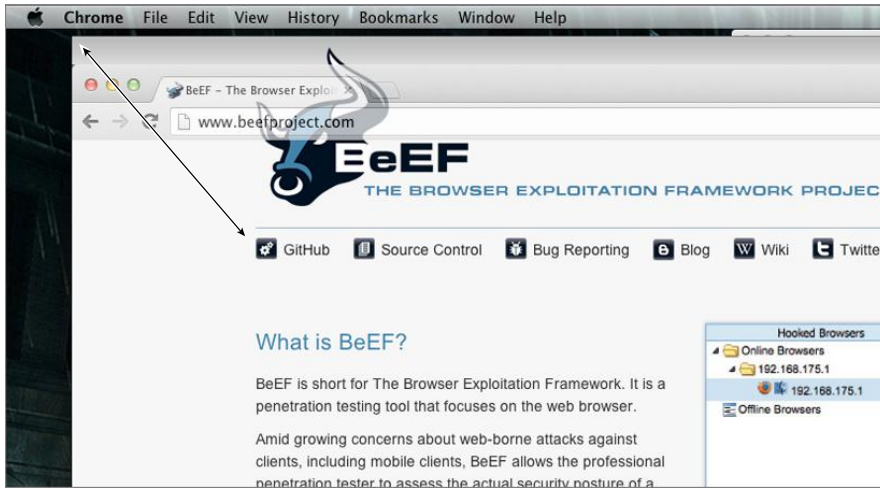
Figure 5-3: Page coordinates
