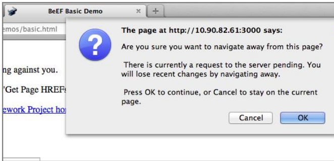
Figure 3-10: First dialog on Firefox 18 with custom content (controlled with JavaScript)
