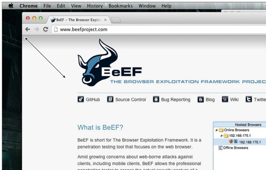
Figure 5-2: Client coordinates
