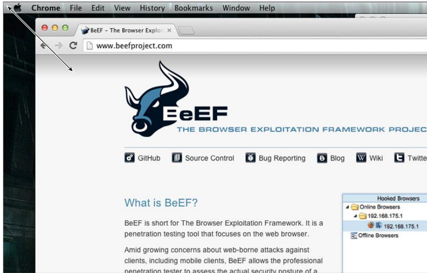
Figure 5-1: Screen coordinates
