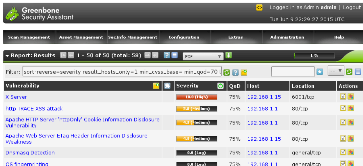
Figure 28 - Vulnerability Count for Our Uncredentialed Scan
