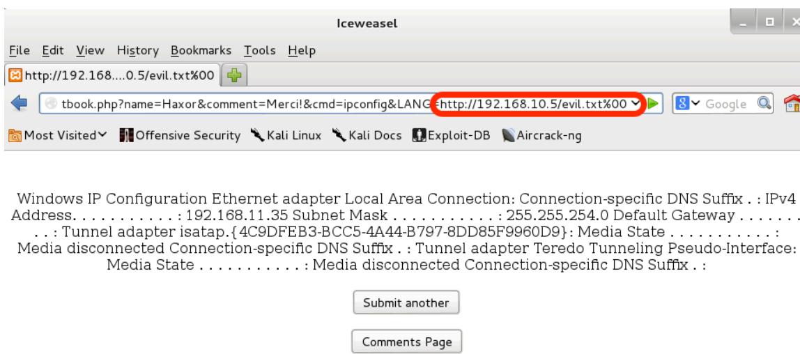
Figure 59 - Exploiting the RFI Vulnerability
