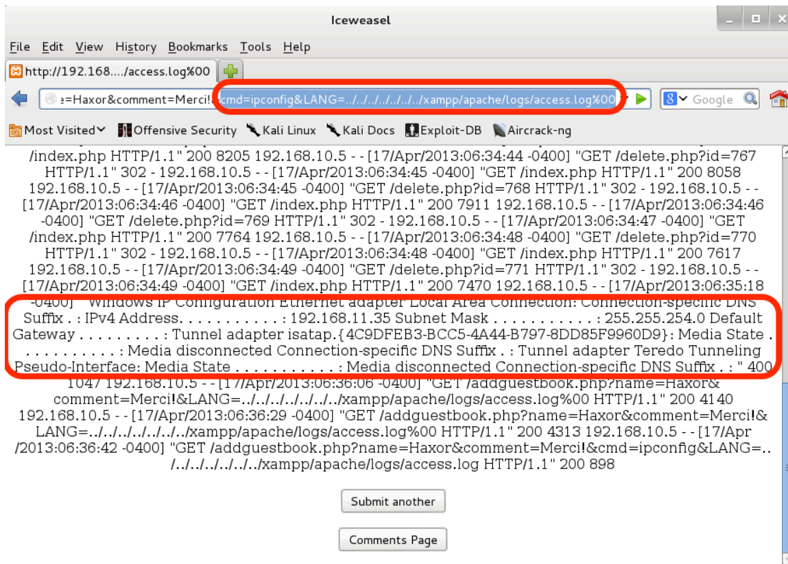
Figure 58 - Executing Code with the LFI Vulnerability
