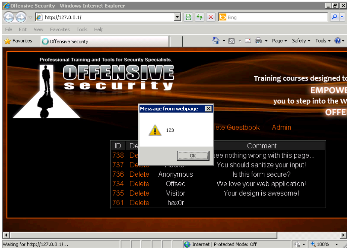
Figure 52 - The JavaScript Executes When the Page is Viewed
