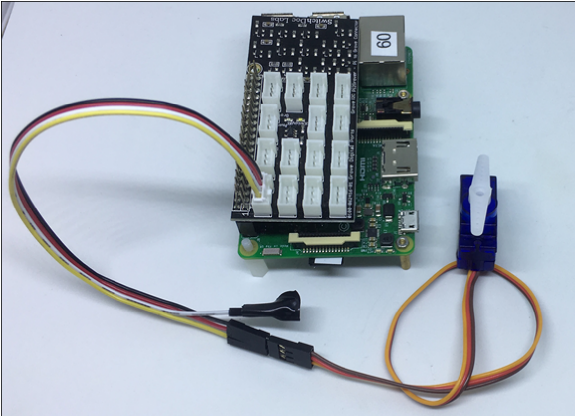
FIGURE 4-12: Fully connected Pi and servo motor.
