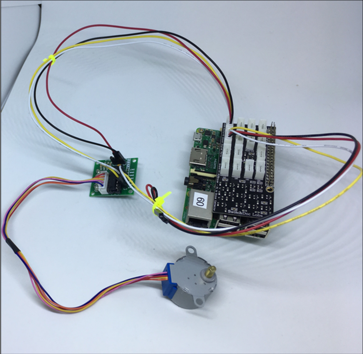
FIGURE 4-21: Fully wired Raspberry Pi and stepper motor project.
