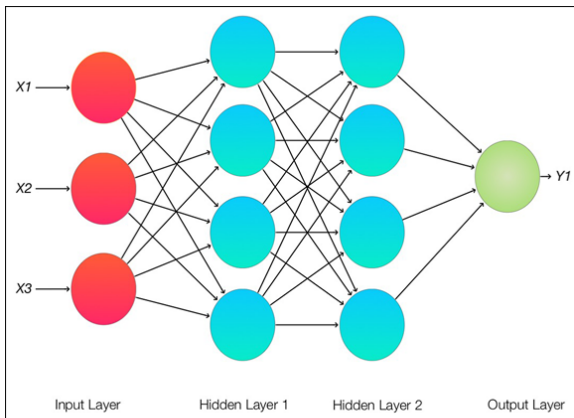
FIGURE 2-5: Our TensorFlow three-layer neural network.
