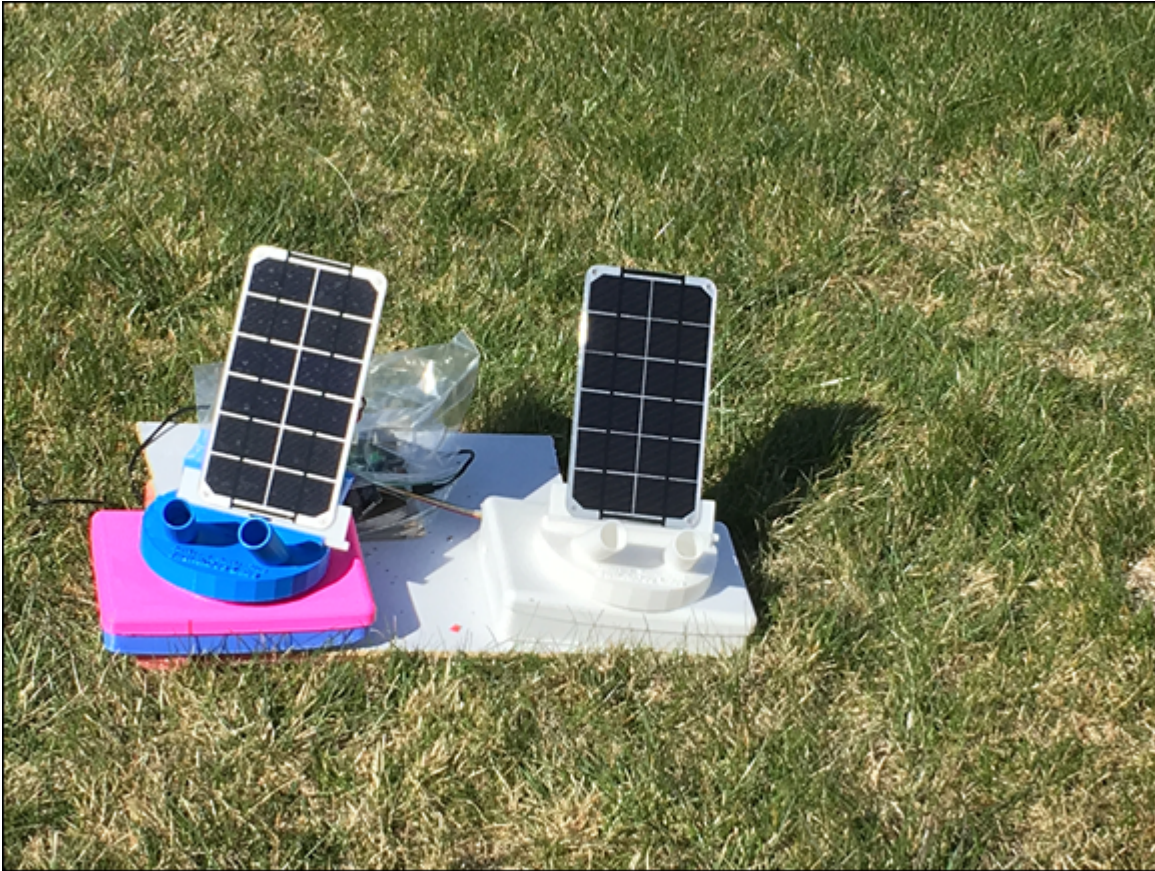
FIGURE 4-2: Sun-tracking solar panels using a stepper motor.
