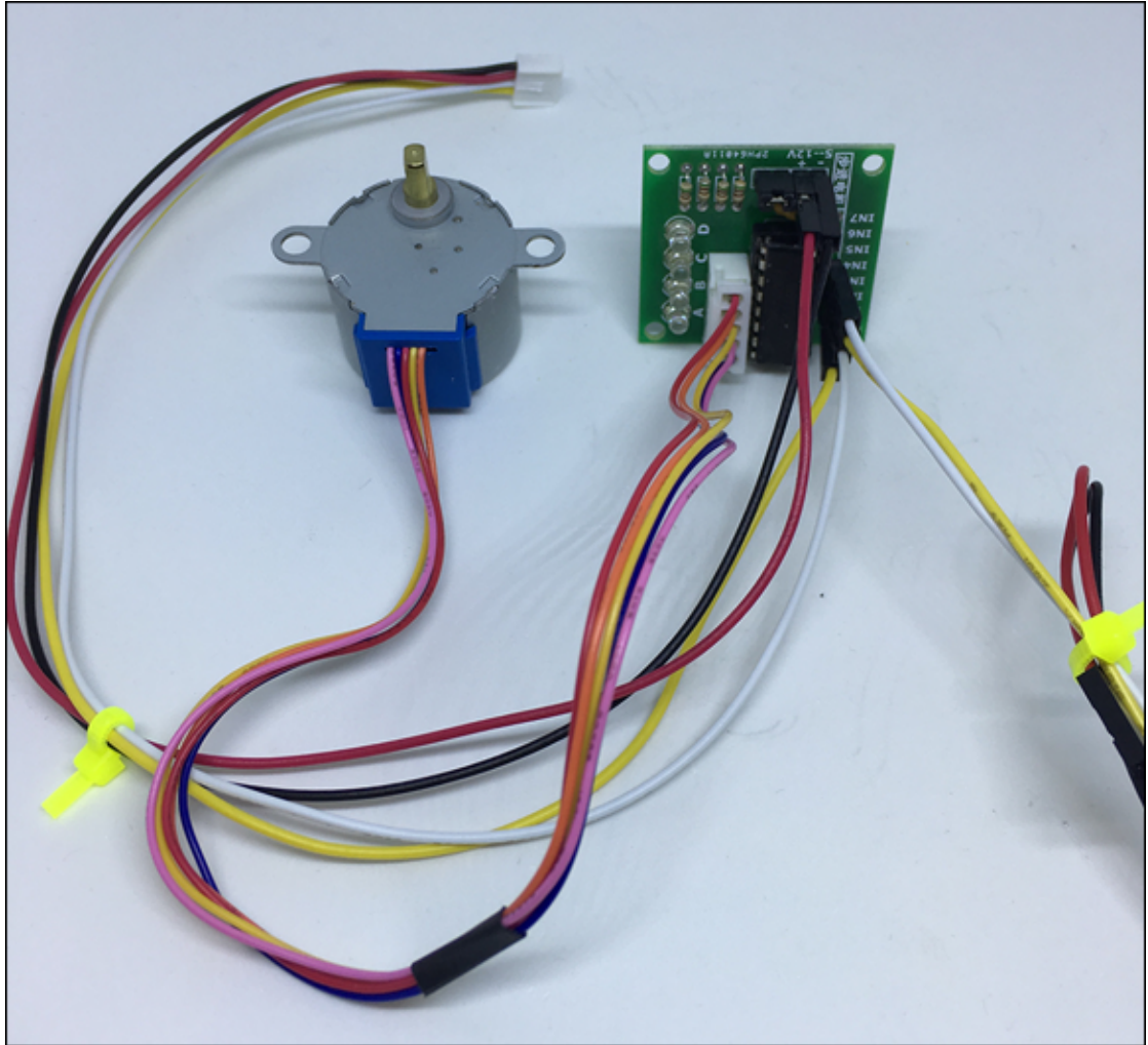
FIGURE 4-20: Stepper motor and driver board connected.
