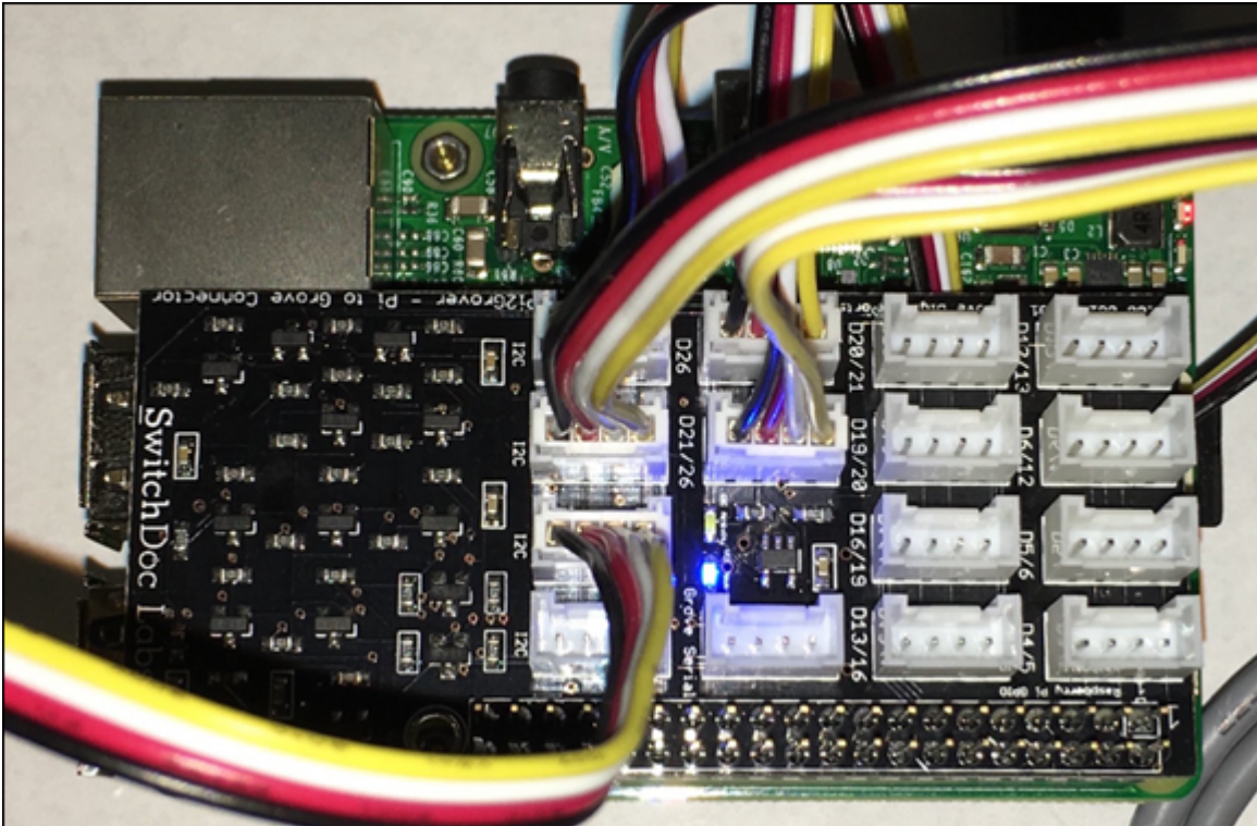
FIGURE 2-3: The Pi2Grover board at work on the Raspberry Pi.
