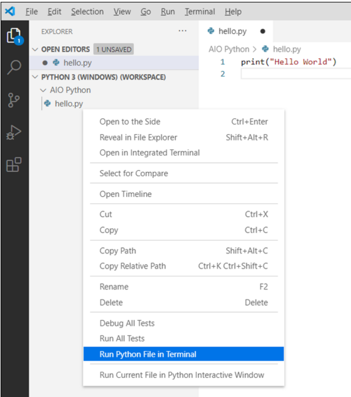
FIGURE 2-14: Run hello.py .
