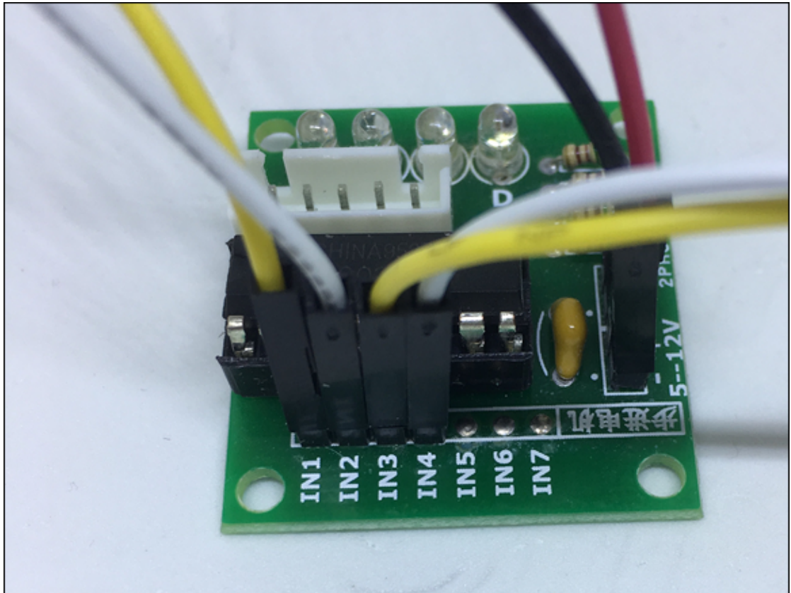
FIGURE 4-19: All patch wires installed on the UNL2003 driver board.
