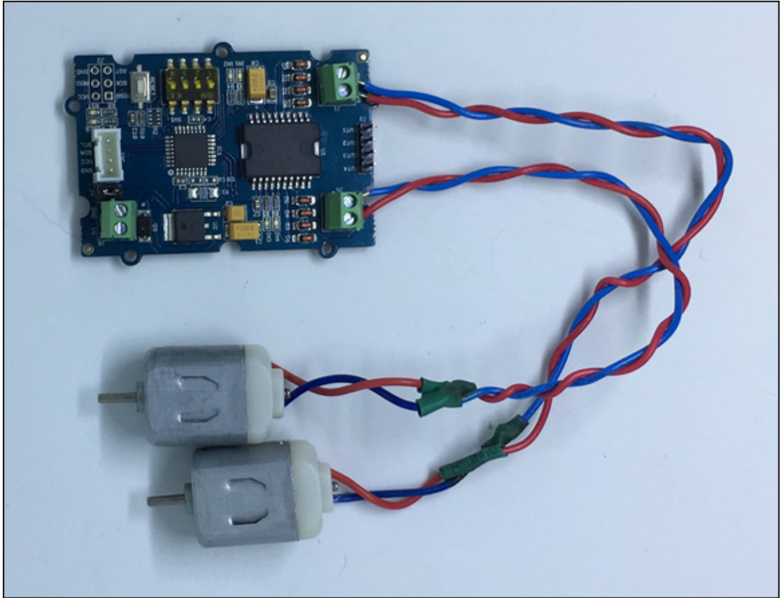
FIGURE 4-7: Motors installed on the motor drive.
