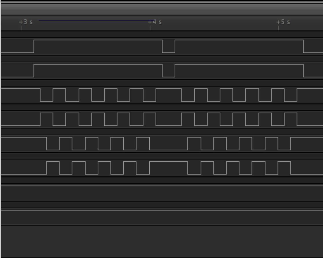
FIGURE 4-14: Logic analyzer showing the motor stepping sequence.
