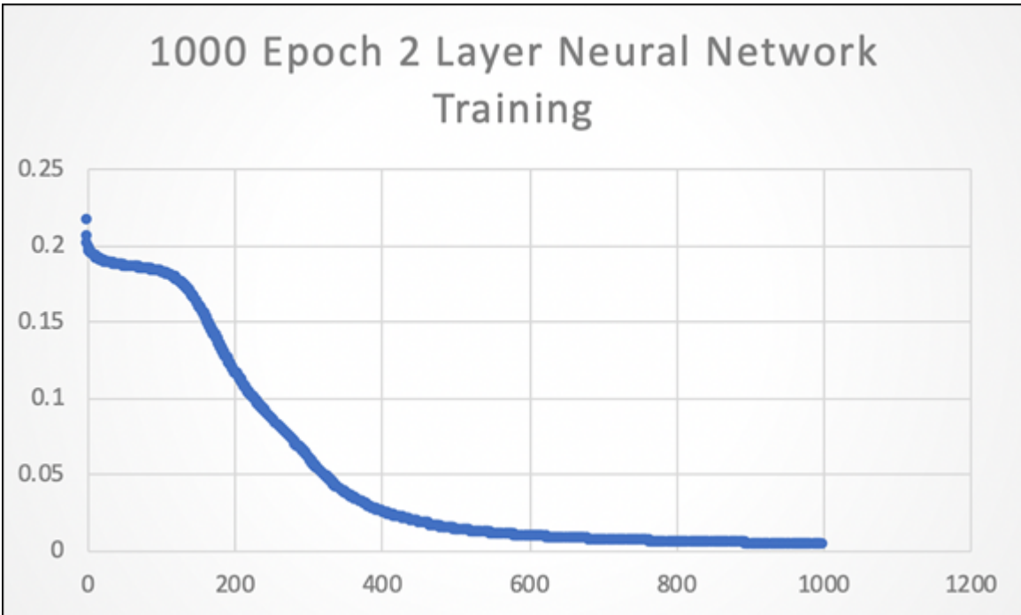
FIGURE 2-4: The Loss function during training.
