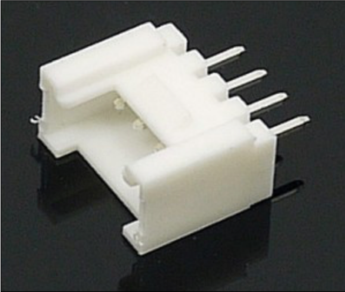
FIGURE 2-4: A Grove connector.
