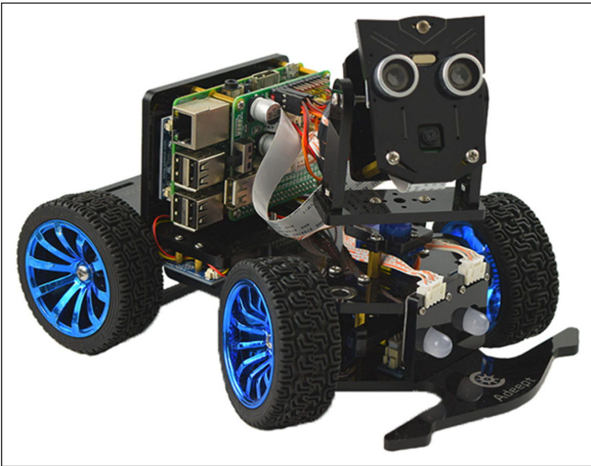
FIGURE 2-10: The assembled PiCar-B showing wiring.
