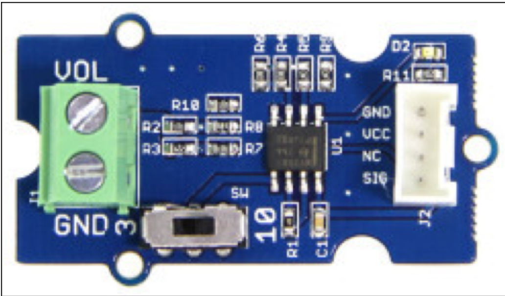
FIGURE 2-7: A Grove analog simple voltage divider.
