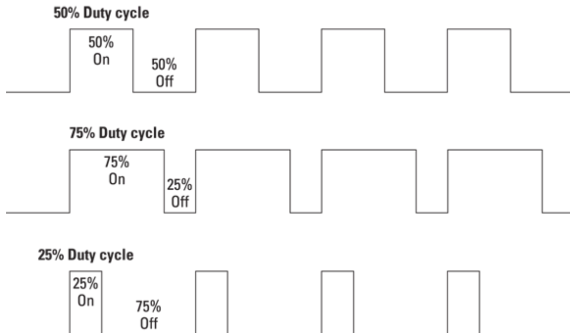
FIGURE 1-10: Duty cycles.
