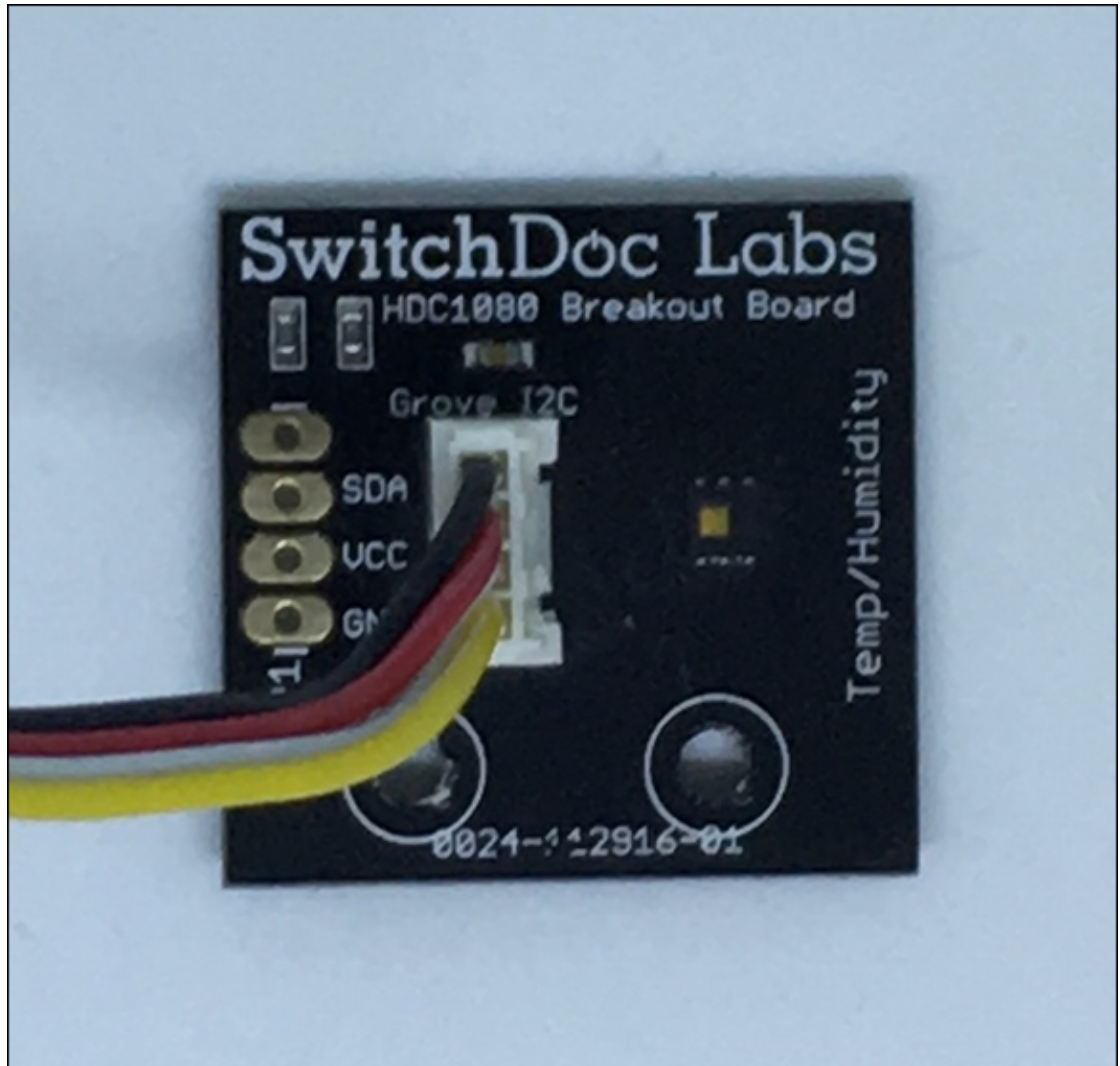
FIGURE 3-3: HDC1080 with the Grove cable plugged in.
