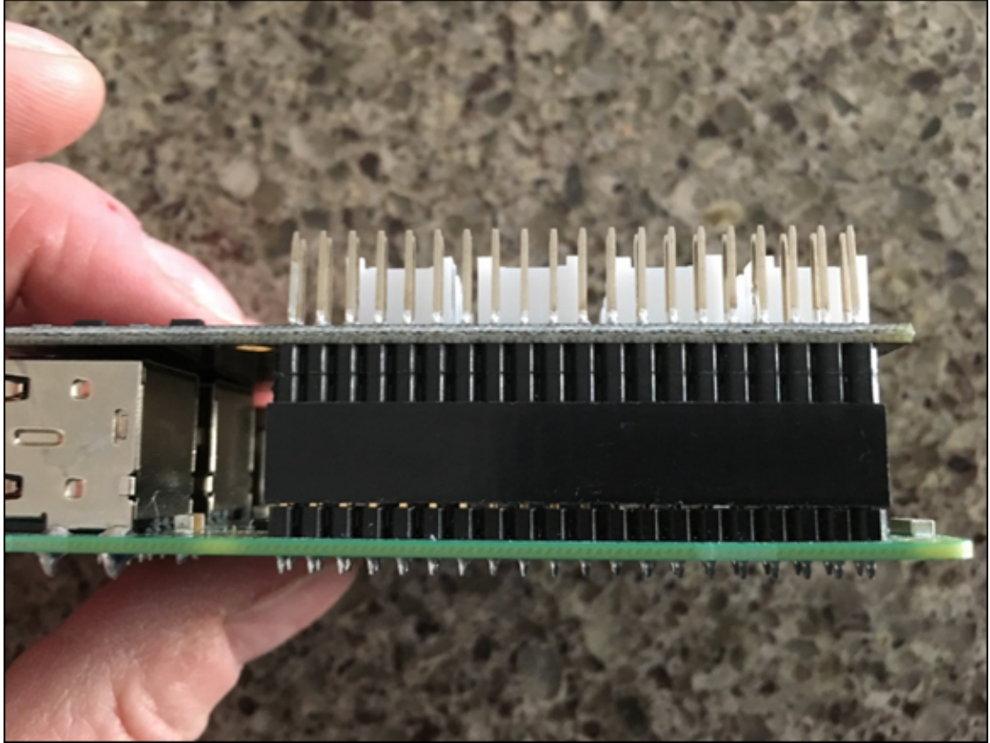
FIGURE 1-6: The installed Pi2Grover board.
