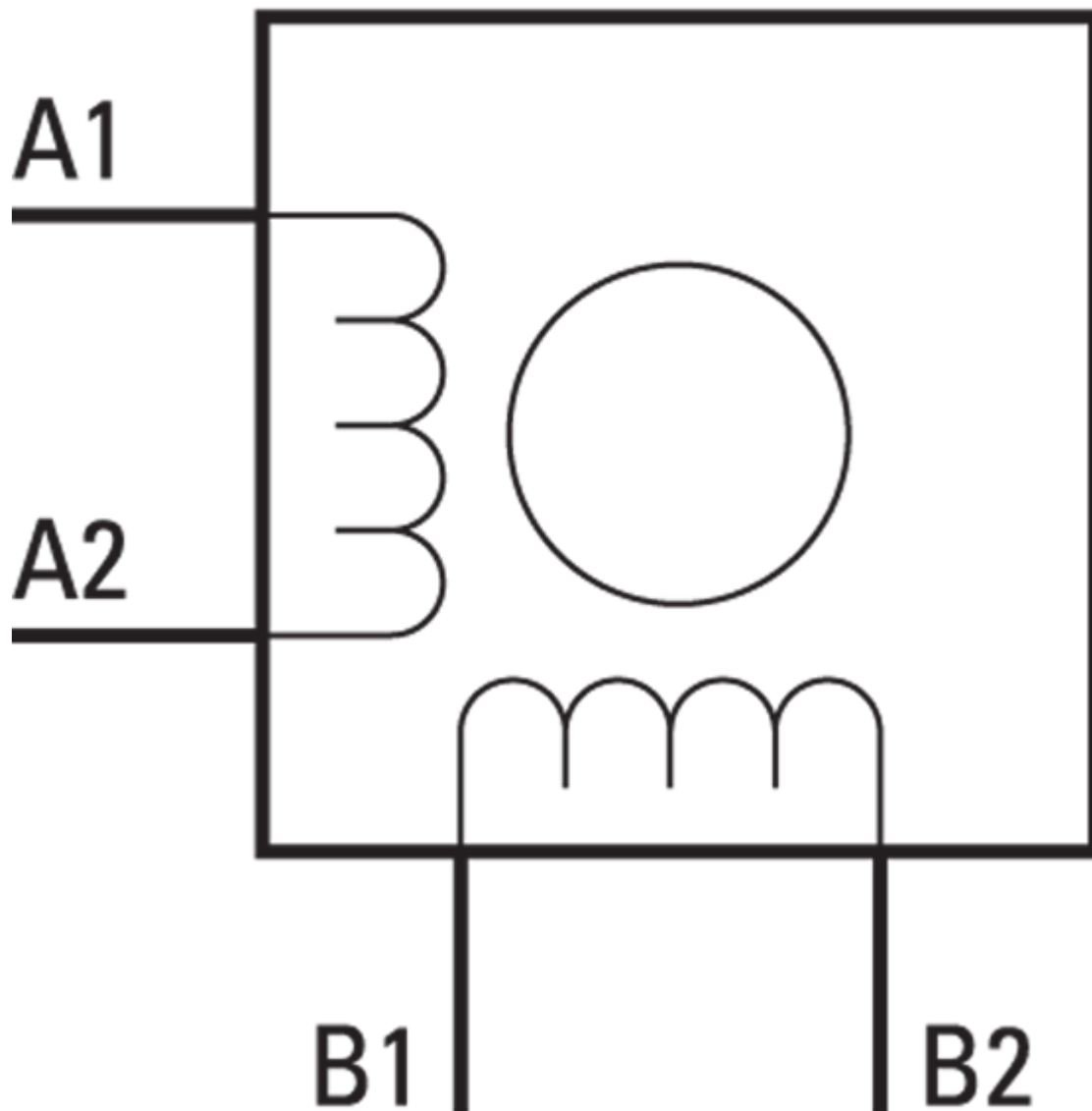
FIGURE 4-13: A diagram of a stepper motor.
