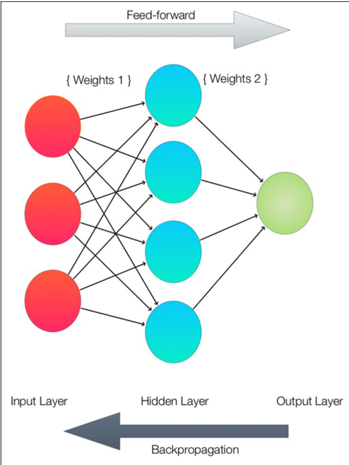
FIGURE 2-2: Feed-forward and backpropagation.
