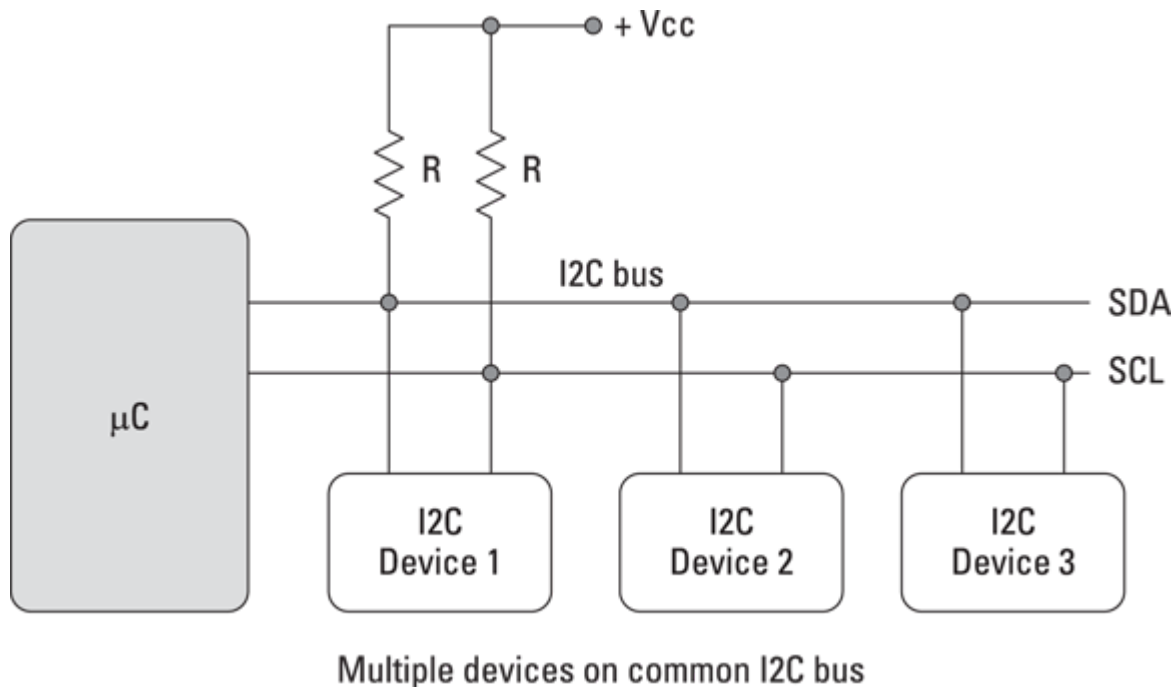
FIGURE 3-1: The I2C bus.
