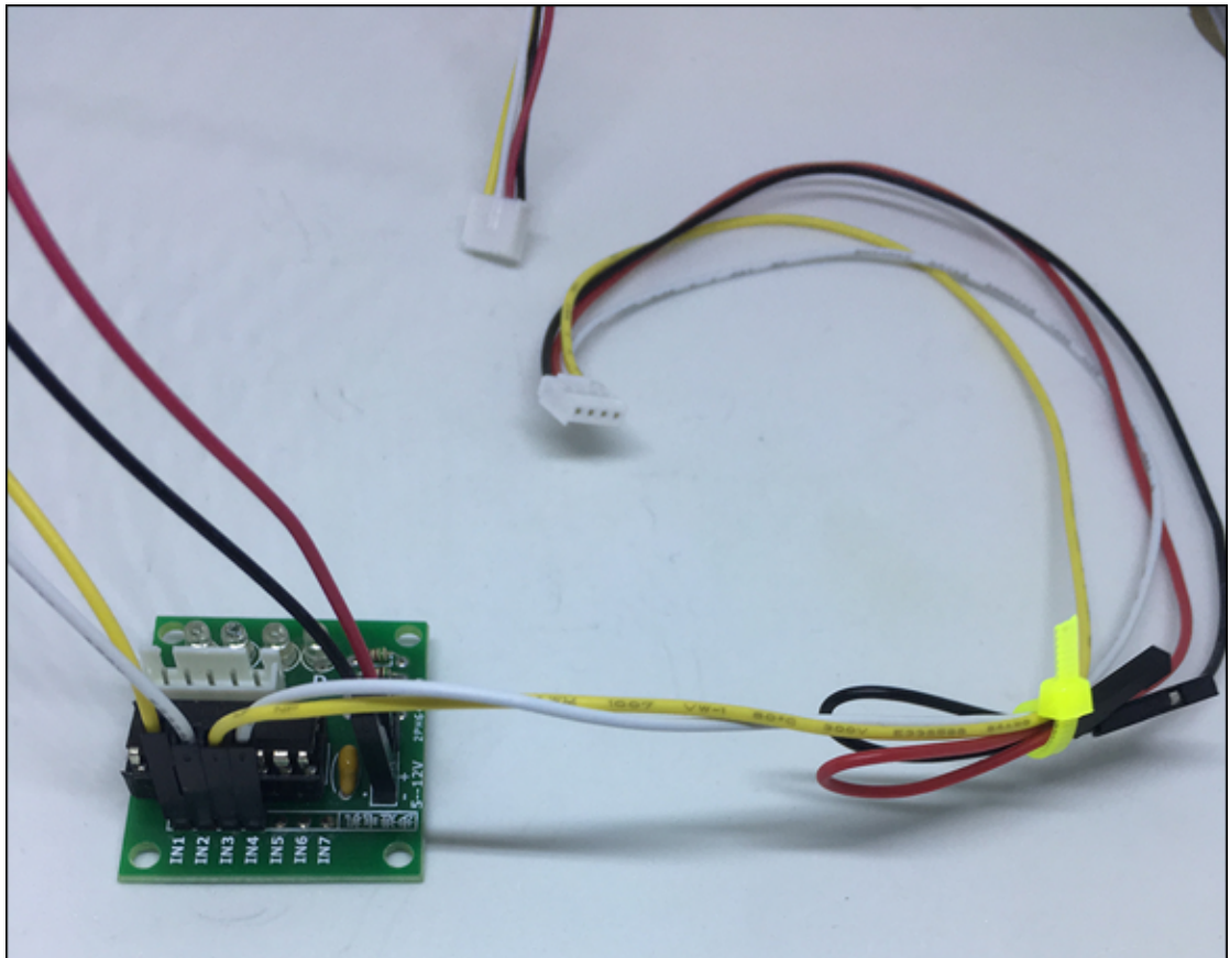
FIGURE 4-18: Second Grove patch cable attached.
