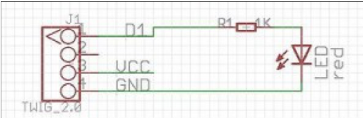
FIGURE 2-6: A simple digital Grove module with LED.
